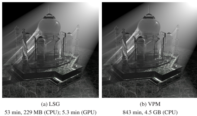
Figure 7: Crystal Taj Mahal. The scene contains 53K triangles and is illuminated by a point light source. Coefficients of the participating medium are \kappa = 0.3 , \sigma = 0.2 . Parameter settings are (a) l = 677K , r = 0.0003 ; (b) p = 64M , knn = 128 , \Delta_x = 0.001 .
